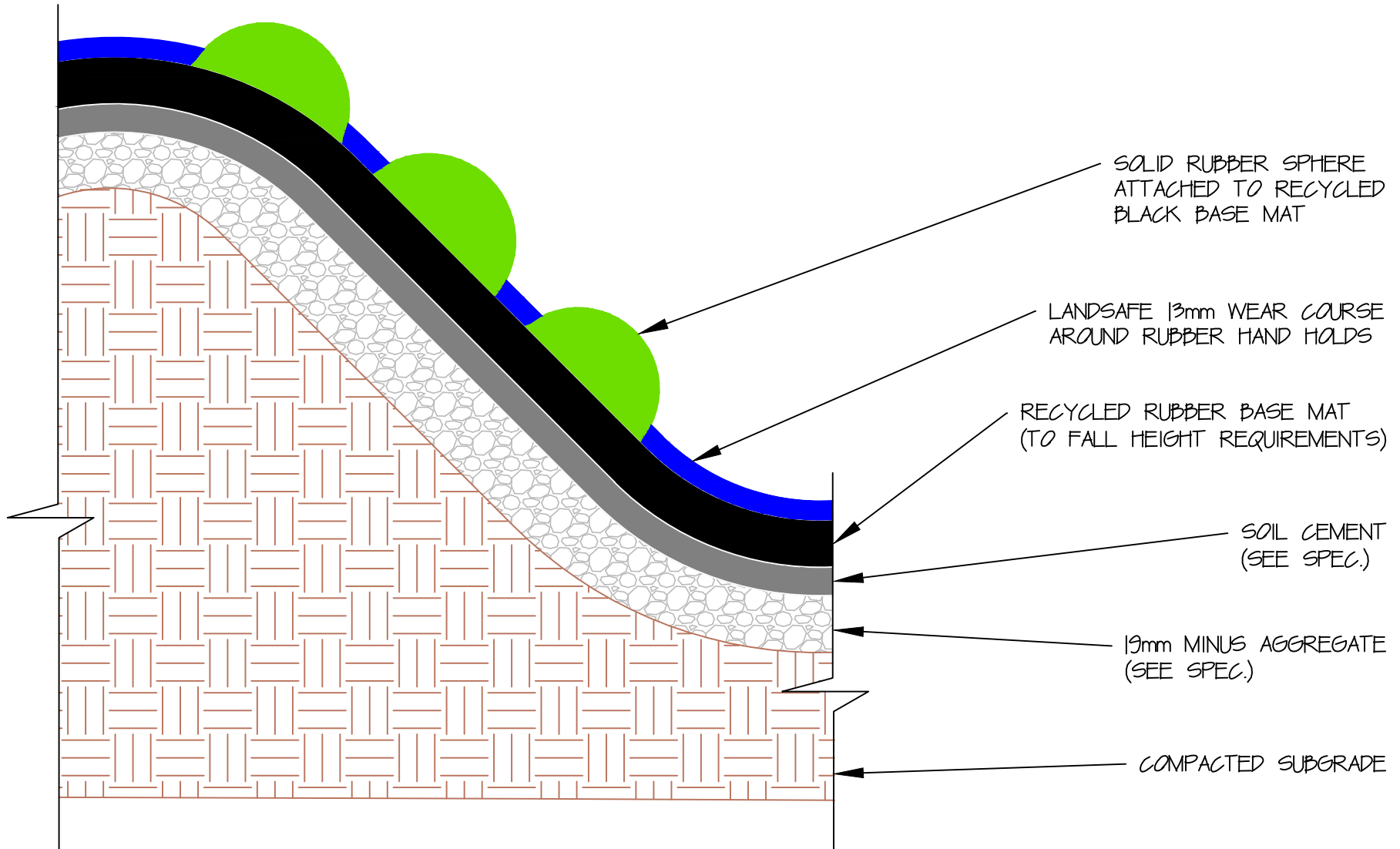
TYPICAL HAND HOLD ON SLOPE SCALE: NTS
