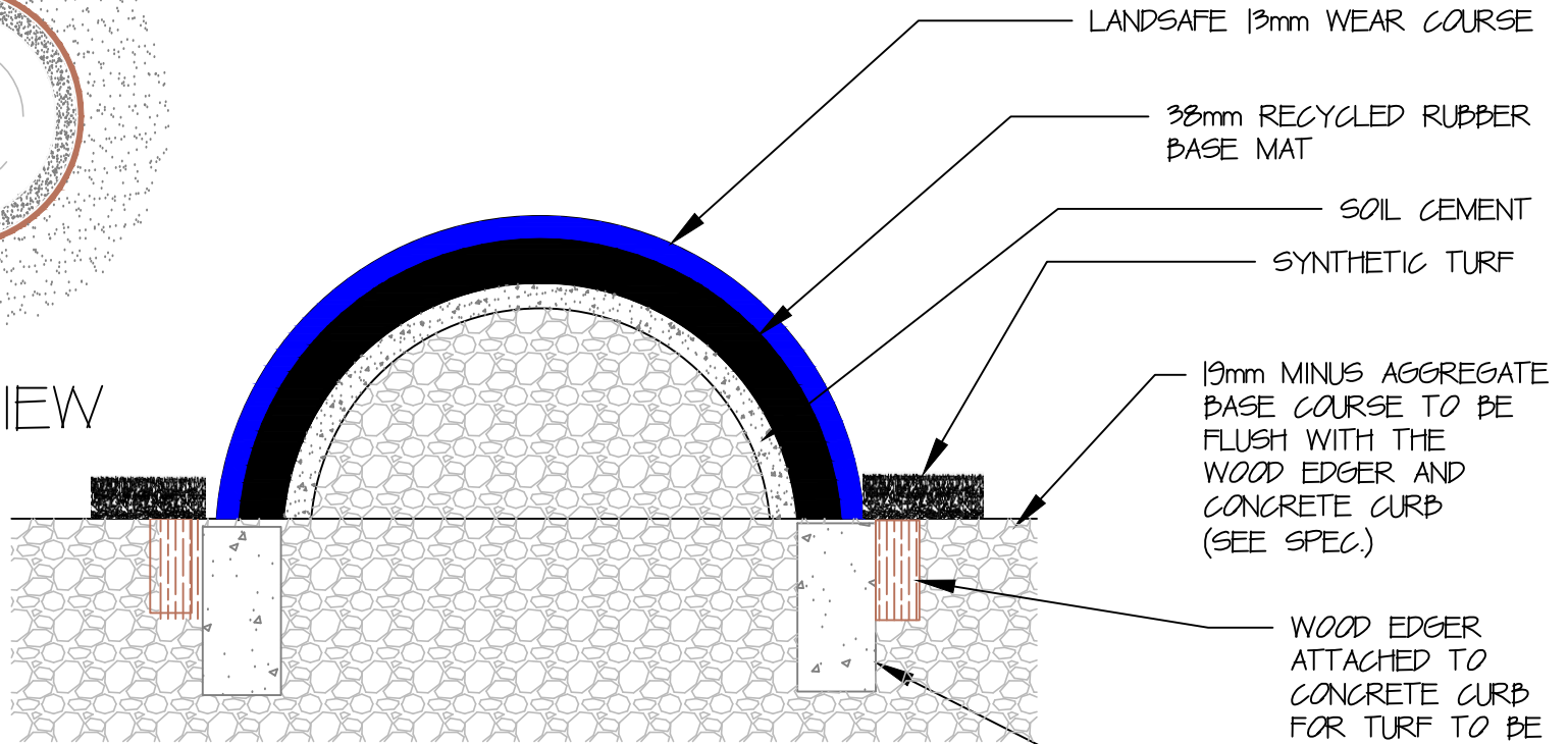
SECTION VIEW
